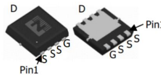
DFN3*3
